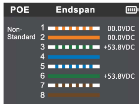
PoE Testing
